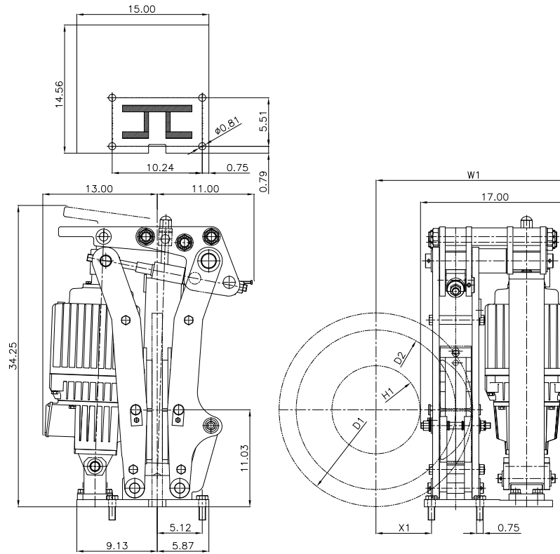
Standard brake designed for 1.18" disc thickness
